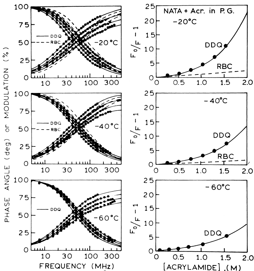
Fig. 4. Left panel: Frequency-domain intensity decays of NATA in propylene glycol in the presence (left to right) concentrations of acrylamide at -20^{\circ}\text{C} (0, 0.512, 1.023 and 1.535 M), at -40^{\circ}\text{C} (0, 0.518, 1.036 and 1.554 M) and at -60^{\circ}\text{C} (0, 0.524, 1.048 and 1.572 M). The solid lines show the best fit to the DDQ model using: (top) a = 5 \text{ \AA} and r_e = 0.317 \text{ \AA} ; (middle) a = 5 \text{ \AA} and r_e = 0.313 \text{ \AA} ; and (bottom) a = 5 \text{ \AA} and r_e = 0.318 \text{ \AA} . The dashed lines show the best fit to the RBC model using a = 5 \text{ \AA} . Right panel: Stern-Volmer plots for NATA quenched by acrylamide in propylene glycol at -20^{\circ}\text{C} , at -40^{\circ}\text{C} and at -60^{\circ}\text{C} . The solid lines represent the calculated values of [(F_0/F) - 1] using parameter values from the DDQ model for a = 5 \text{ \AA} . The dashed lines represent the RBC model using also a = 5 \text{ \AA} .
