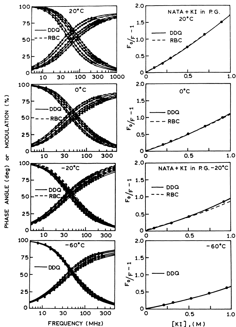
Fig. 7. Left panel: Frequency-domain intensity decays of NATA in propylene glycol in the presence (left to right) concentrations of iodide at 20°C (0, 0.2, 0.5, 0.7 and 0.9 M), 0°C (0, 0.202, 0.505, 0.707 and 0.909 M), -20°C (0, 0.205, 0.512, 0.716 and 0.921 M), and -60°C (0, 0.210, 0.524, 0.734 and 0.943 M). The solid lines show the best fit to the DDQ model using from (top to bottom) a = 5 \text{ \AA} and r_c = 0.623 \text{ \AA} , 0.631 \text{ \AA} , 0.557 \text{ \AA} and 0.513 \text{ \AA} , correspondingly. The dashed lines show the best fit to the RBC model using a = 5 \text{ \AA} . Right panel: Stern-Volmer plots for NATA quenched by iodide in propylene glycol at 20°C, 0°C, -20°C and -60°C. The solid lines represent the calculated values of [(F_0/F) - 1] using parameter values from the DDQ model for a = 5 \text{ \AA} . The dashed lines represent the RBC model using also a = 5 \text{ \AA} .
