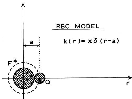
Scheme 1. RBC model for collisional quenching of fluorescence.
