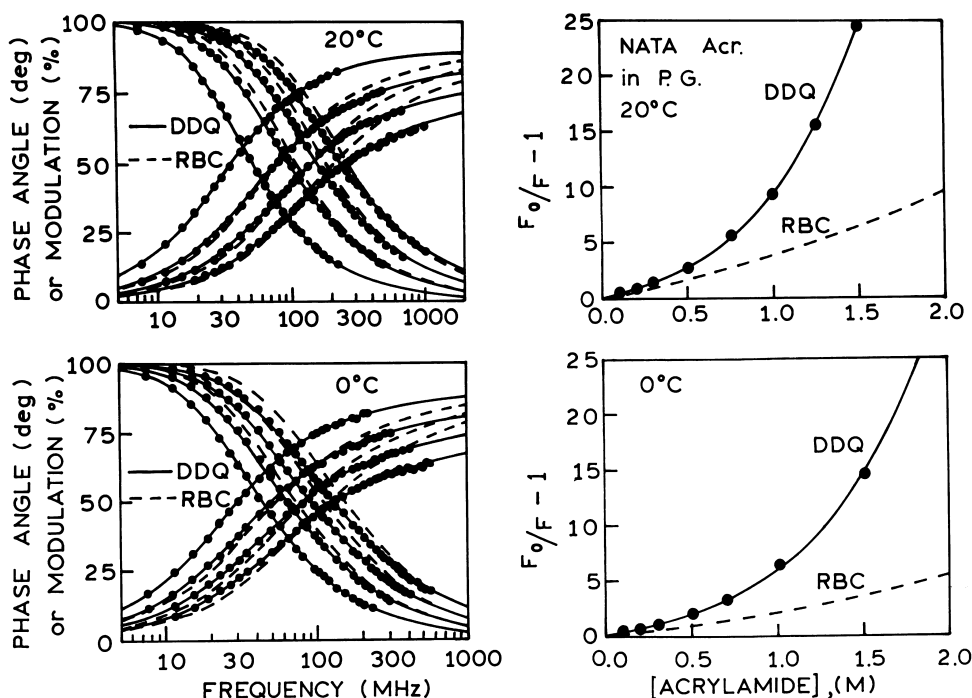
Fig. 3. Left panel: Frequency-domain intensity decays of NATA in propylene glycol in the presence (left to right) concentration of acrylamide at 20°C (0, 0.5, 1.0 and 1.5 M) and at 0°C (0, 0.505, 1.010 and 1.515 M). The solid lines show the best fit to the DDQ model using: (upper) a = 5 \text{ \AA} and r_e = 0.322 \text{ \AA} ; and (lower) a = 5 \text{ \AA} and r_e = 0.318 \text{ \AA} . The dashed lines show the best fit to the RBC model using a = 5 \text{ \AA} . Right panel: Stern–Volmer plots for NATA quenched by acrylamide in propylene glycol at 20°C and at 0°C. The solid lines represent the calculated values of [(F_0/F) - 1] using parameter values from the DDQ model for a = 5 \text{ \AA} . The dashed lines represent the RBC model using also a = 5 \text{ \AA} .
