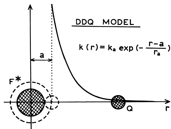
Scheme 2. DDQ model for collisional quenching of fluorescence.
